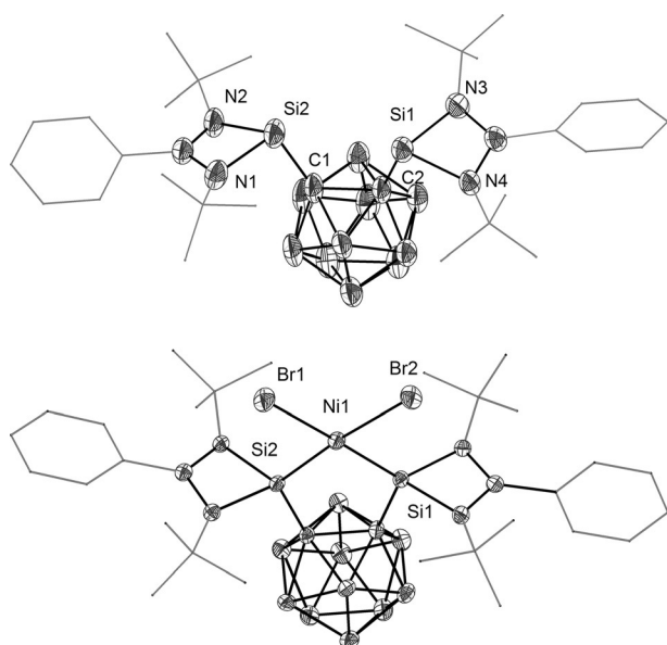
Figure 1. Molecular structure of \text{SiCCSi} (top) and [\text{SiCCSi}]\text{NiBr}_2 (bottom). Thermal ellipsoids are set at 50% probability. Hydrogen atoms and solvent molecules are omitted for clarity.
