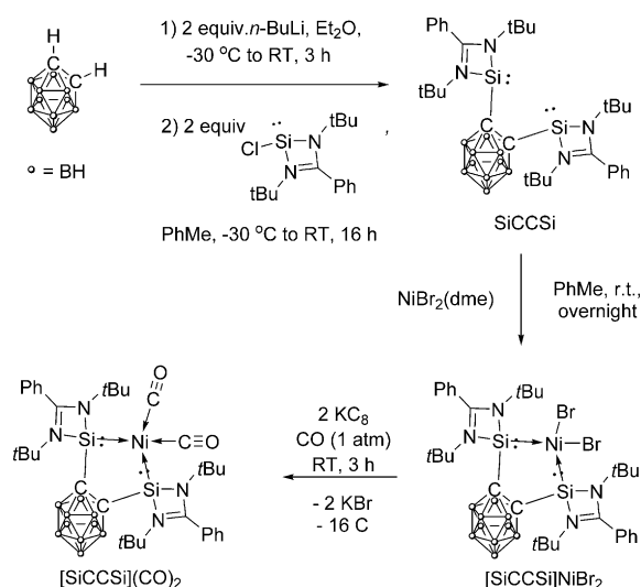
Scheme 2. Synthesis of the [\text{SiCCSi}]\text{NiBr}_2 and [\text{SiCCSi}]\text{Ni}(\text{CO})_2 complexes.
